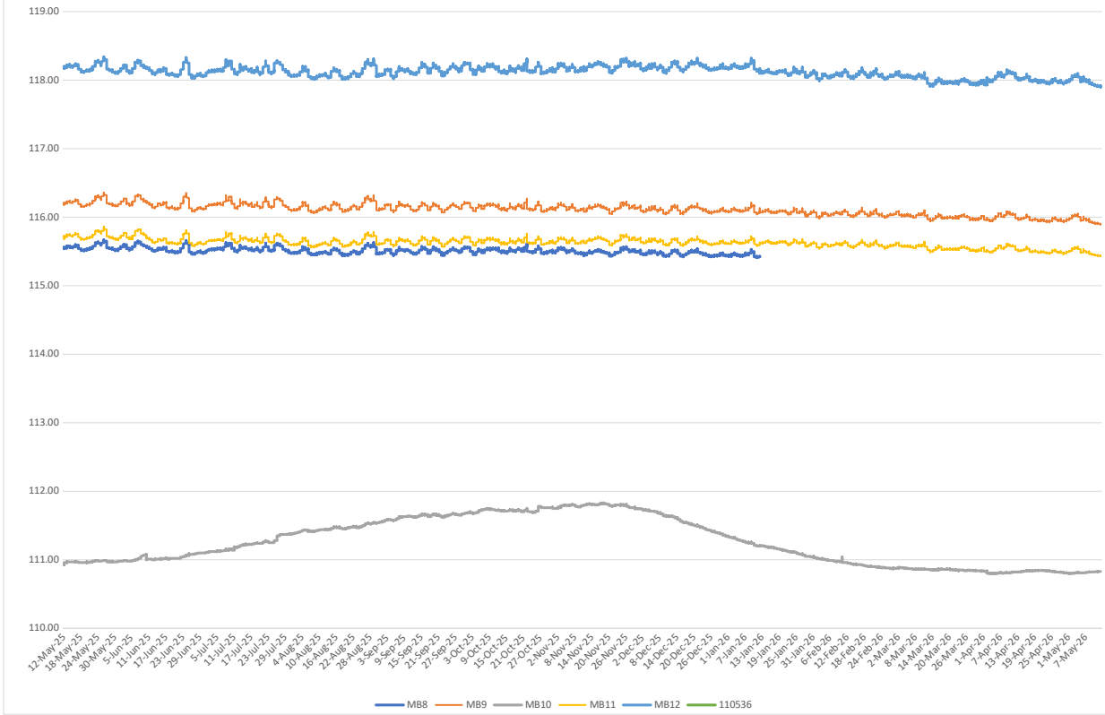
Bore Hydrographs 12 May 2025 - 12 May 2026
